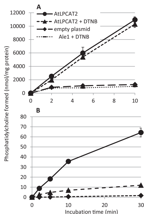
FIGURE 1. Time course of [ ^{14}\text{C} ]18:1 incorporation from [ ^{14}\text{C} ]18:1-CoA into PC in microsomal preparations of the ale1 yeast strain expressing AtLPCAT2. A, incorporation of [ ^{14}\text{C} ]18:1 into PC in the presence of added LPC (forward reaction). B, incorporation of [ ^{14}\text{C} ]18:1 into PC in the absence of LPC with added BSA and free CoA (incorporation via acyl exchange). Incubation conditions as assays for forward reaction (A) and reverse reaction without addition of LPC (B) (see "Experimental Procedures") are shown. The DTNB concentration was 5 mM. Assays were performed in duplicate, and error bars are given \pm S.D.
